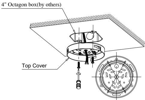
3. Mounting the top cover onto the J-box.
