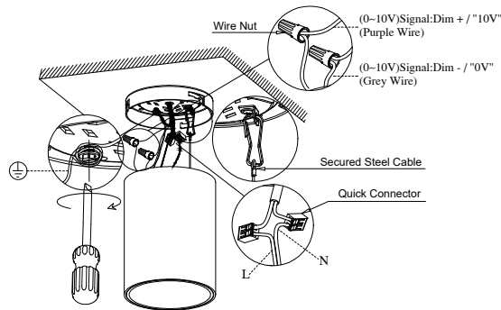
4. Making all the wire connections as the drawing shown.
