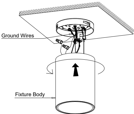
5. Mounting the fixture body to the top cover by counterclockwise rotation until no more force can be exerted.
