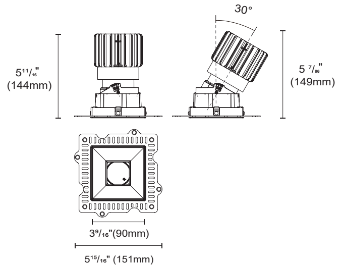
Square Bevel Trimless Adjustable
