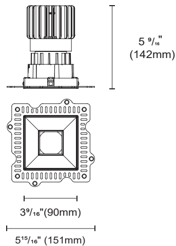
Square Bevel Trimless Fixed
