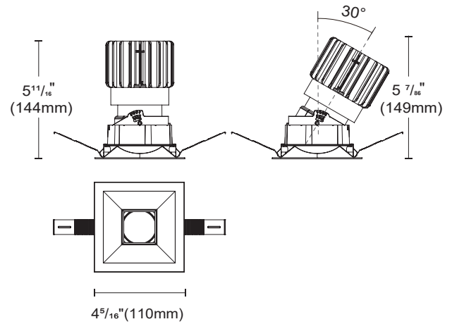
Square Bevel Trim Adjustable
