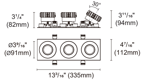
Round Bevel Trim Adjustable- Three Light
