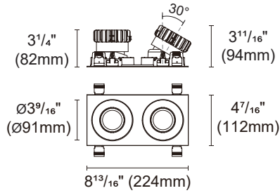
Round Bevel Trim Adjustable- Two Light
