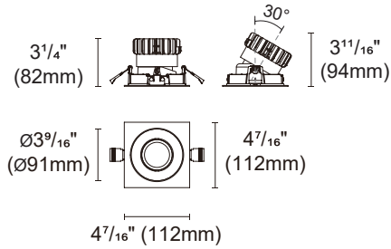
Round Bevel Trim Adjustable- One Light
