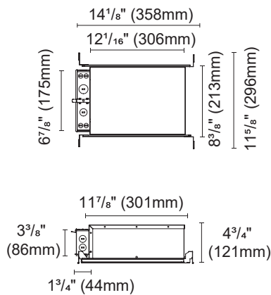
IC BOX For Single Light Upto 14W
