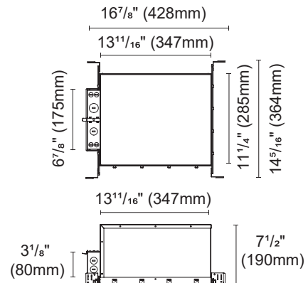
IC BOX For Single Light For 21W
